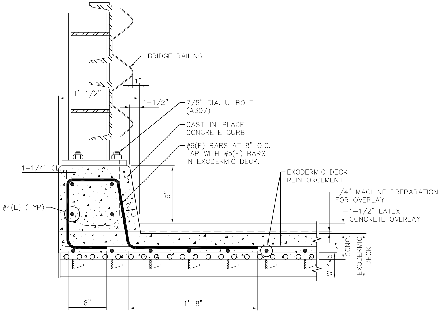
CURB AND BRIDGE RAIL DETAIL
